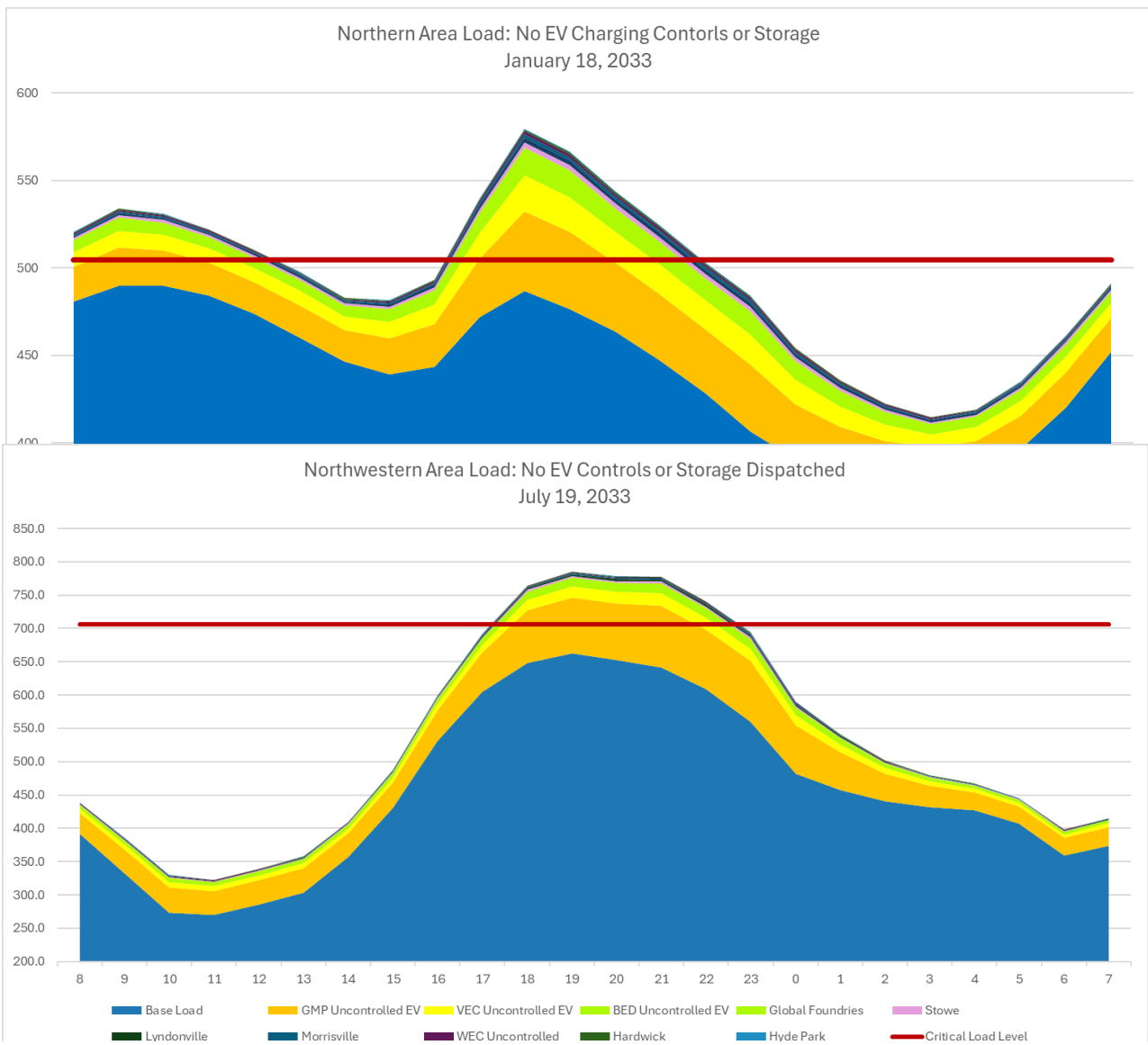
FIGURE 1: NORTHWESTERN VERMONT AREA LOADS ON THE PEAK SUMMER DAY IN 2033. THERE ARE NO EV CONTROLS OR STORAGE APPLIED IN THIS GRAPH, CONSISTENT WITH THE ORIGINAL ASSUMPTIONS MADE IN THE 2024 LONG RANGE TRANSMISSION PLAN.
